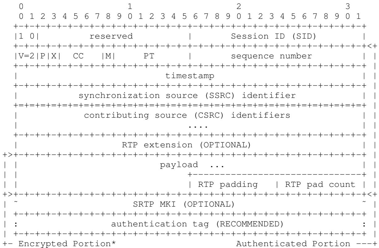
Figure 4: SRTP Packet encapsulated by Session ID Layer
