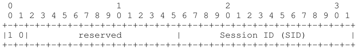
Figure 3: Session ID layer shim header
