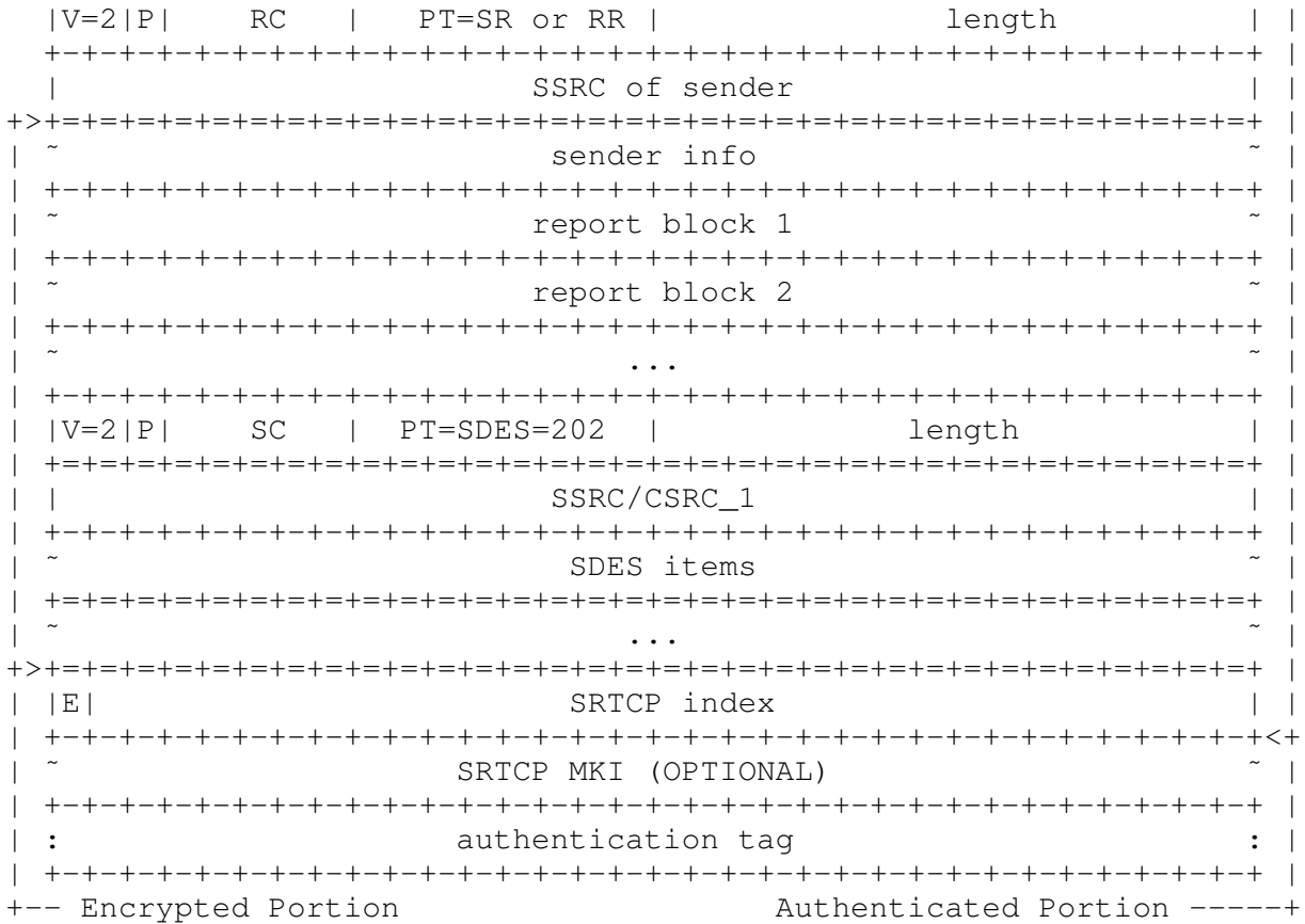
Figure 5: SRTCP packet encapsulated by Session ID layer
