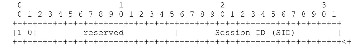
Figure 4: SRTP Packet encapsulated by Session ID Layer
