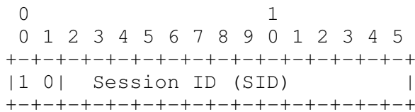
Figure 2: Session ID layer
