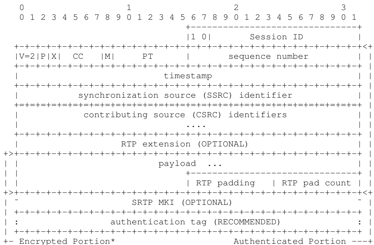
Figure 3: SRTP Packet encapsulated by Session ID Layer
