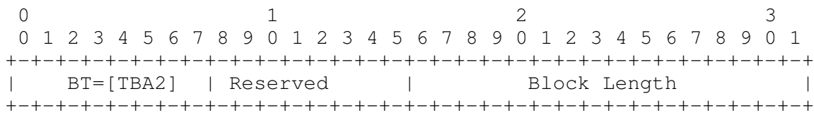
Figure 3: RTCP XR Report Header
