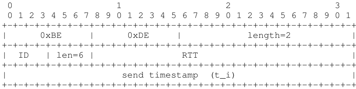
Figure 1: RTP Sender Header Extension Block
