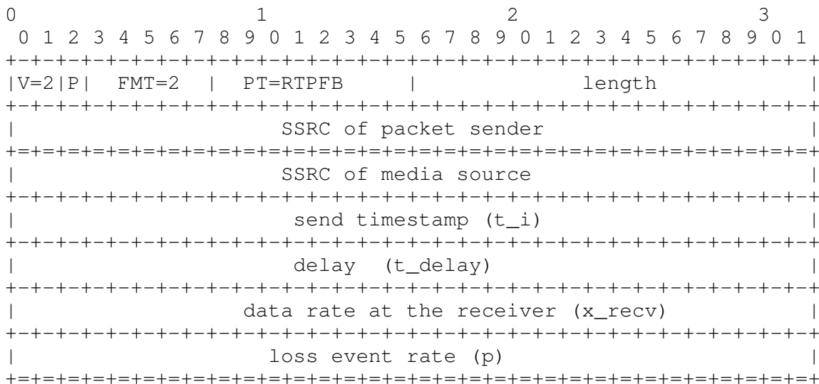
Figure 2: The AVPF TFRC-FB RTCP Transport Layer Feedback Message
