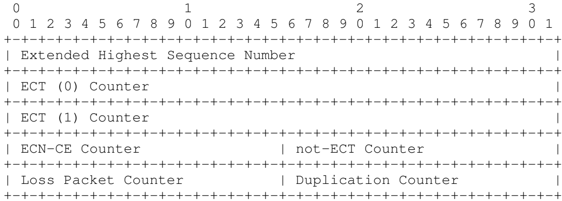
Figure 2: ECN Feedback Report Format
