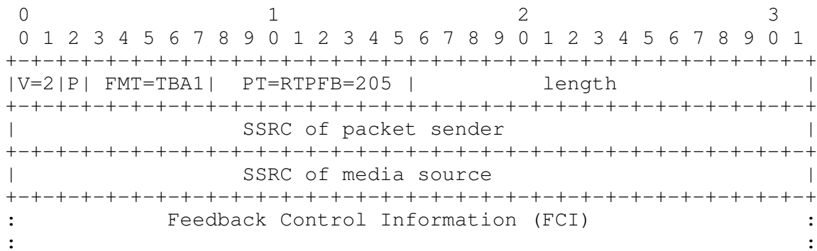
Figure 1: RTP/AVPF Common Packet Format for Feedback Messages
