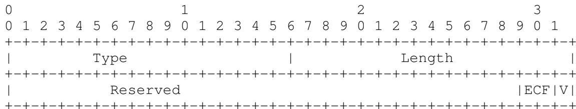
Figure 6: ECN Check STUN Attribute
