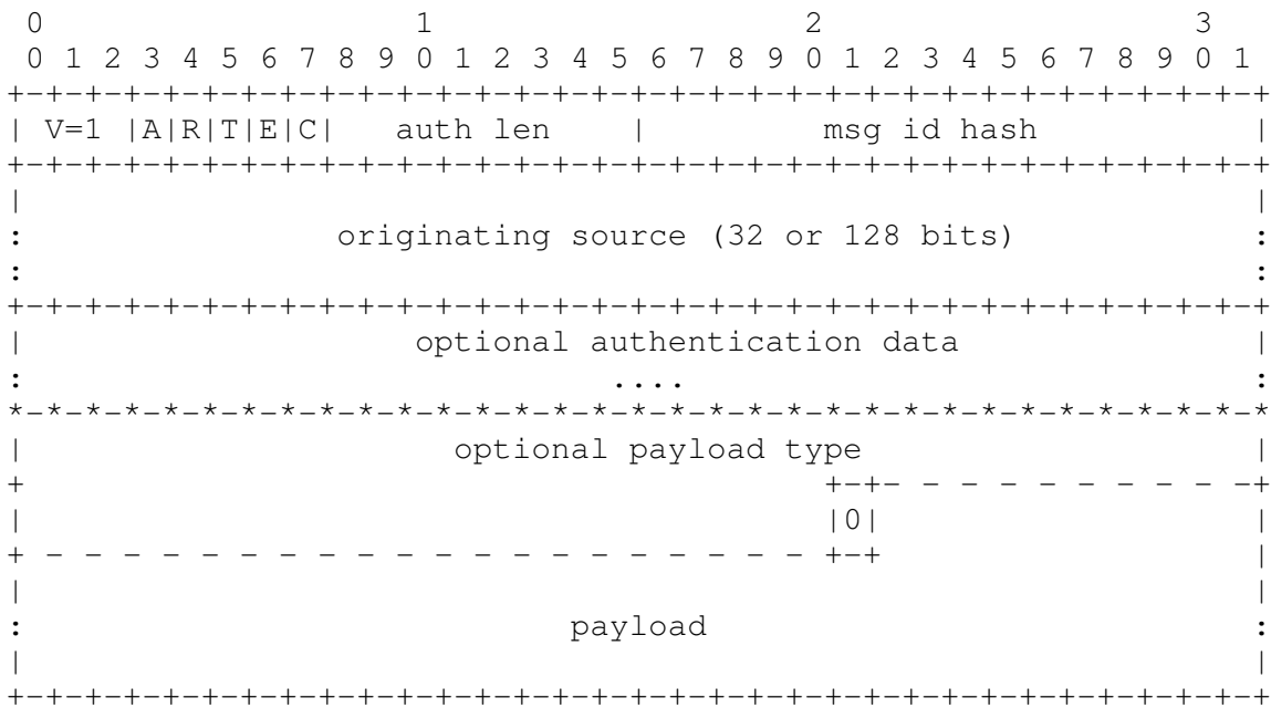
Figure 1: Packet format
