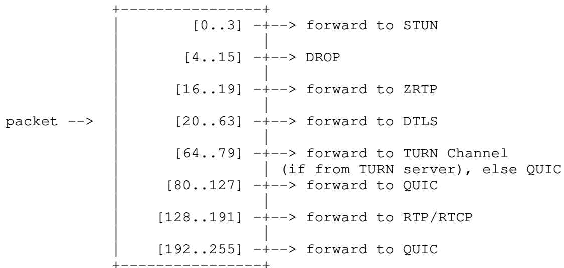
Figure 3: The receiver's packet demultiplexing algorithm.
