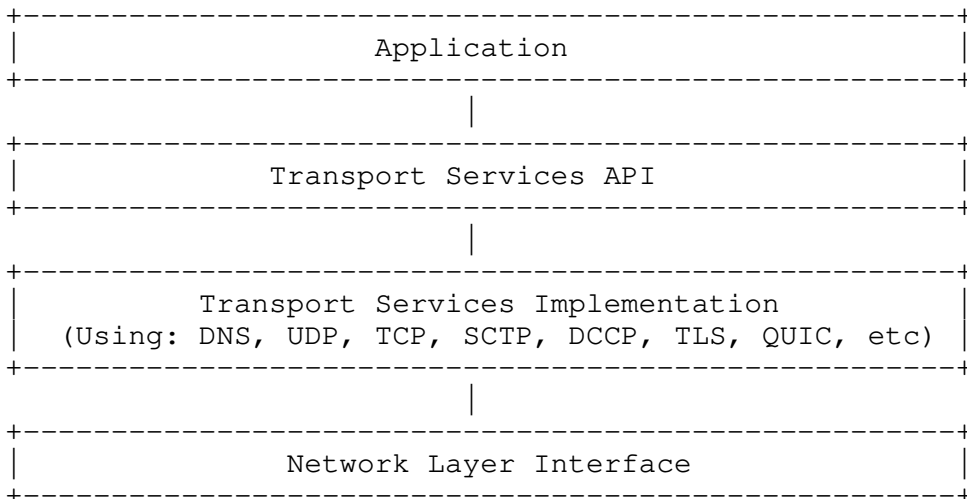
Figure 2: Transport Services API Model
