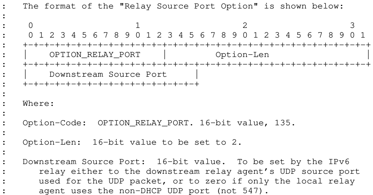
Figure 3: DHCPv6's Relay Source Port Option (from [RFC8357])
